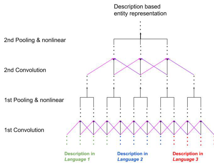
Fig. 2: Passing pre-trained multilingual word embeddings to a CNN encoder which is adopted from DKRL [15], in order to encode multilingual entity descriptions.
