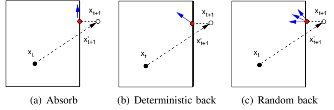
Fig. 1. Different methods to modify velocity settings for a particle relocated onto the border.
