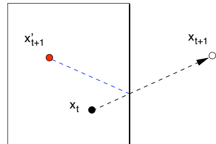
Fig. 5. The Reflect Method. The particle violates the horizontal border and the new position is relected in the search space even farther to the border than before.
