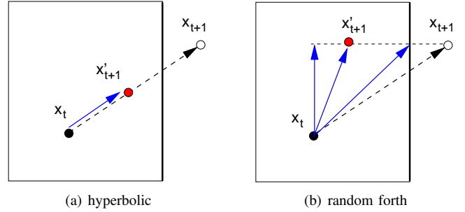
Fig. 2. Boundary handling methods which always keep the particles inside the feasible area.
