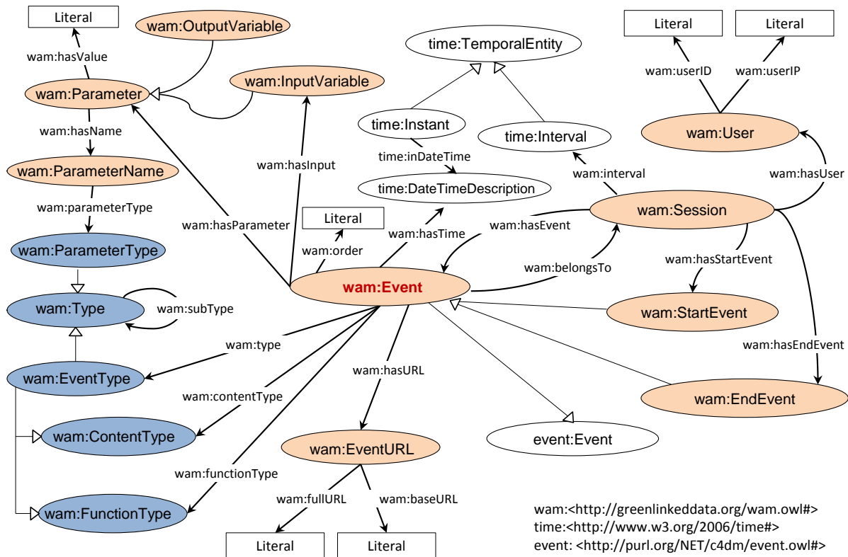
Figure 2: WAM Ontology
