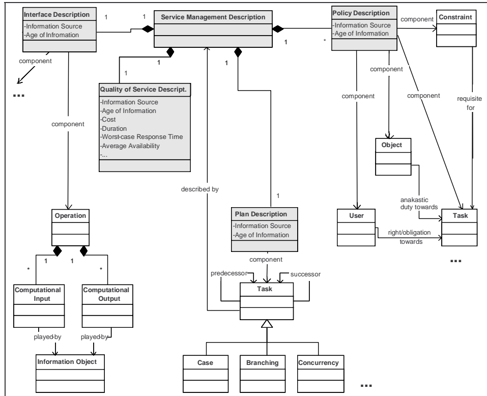
Figure 1: Sketch of the Core Ontology of Services 2
