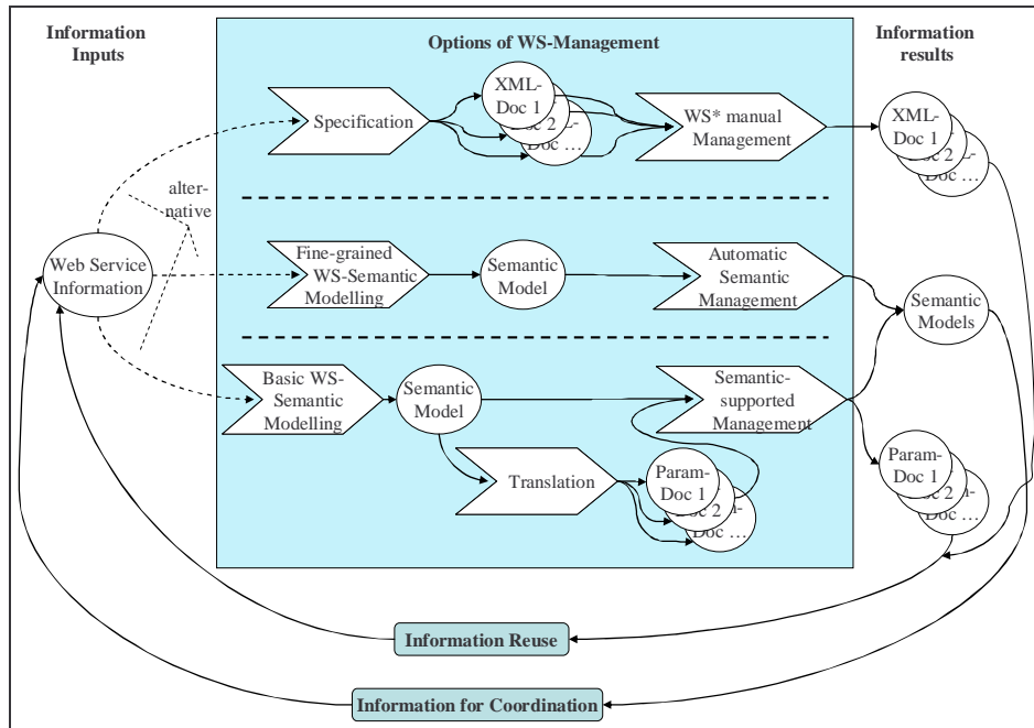
Figure 3: Necessary Information for Development and Management of Web Services
